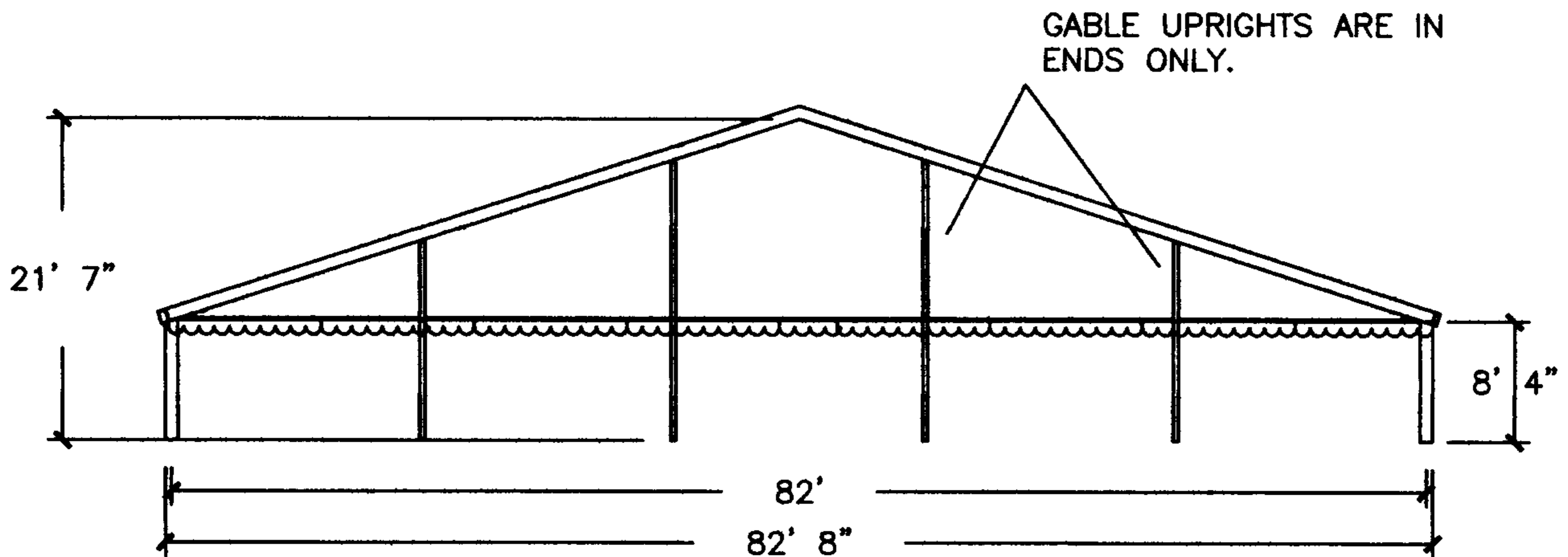
CROSS SECTION
