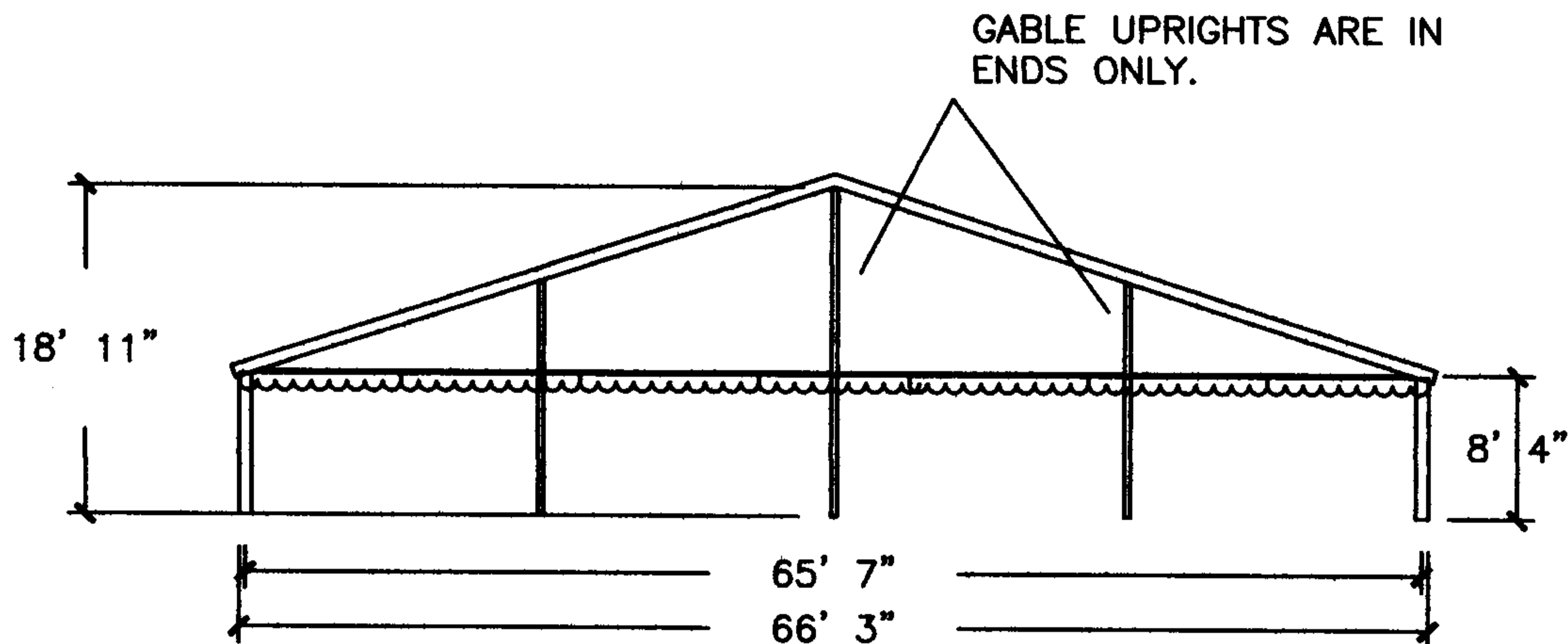
CROSS SECTION
